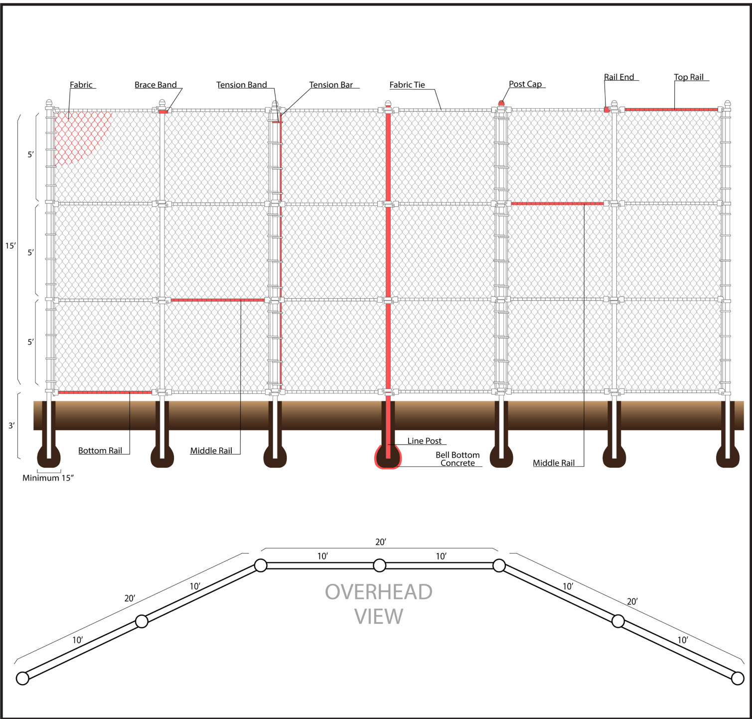
Baseball Fence Backstop Kit 15' High x 20' Wide x 20' Wings
